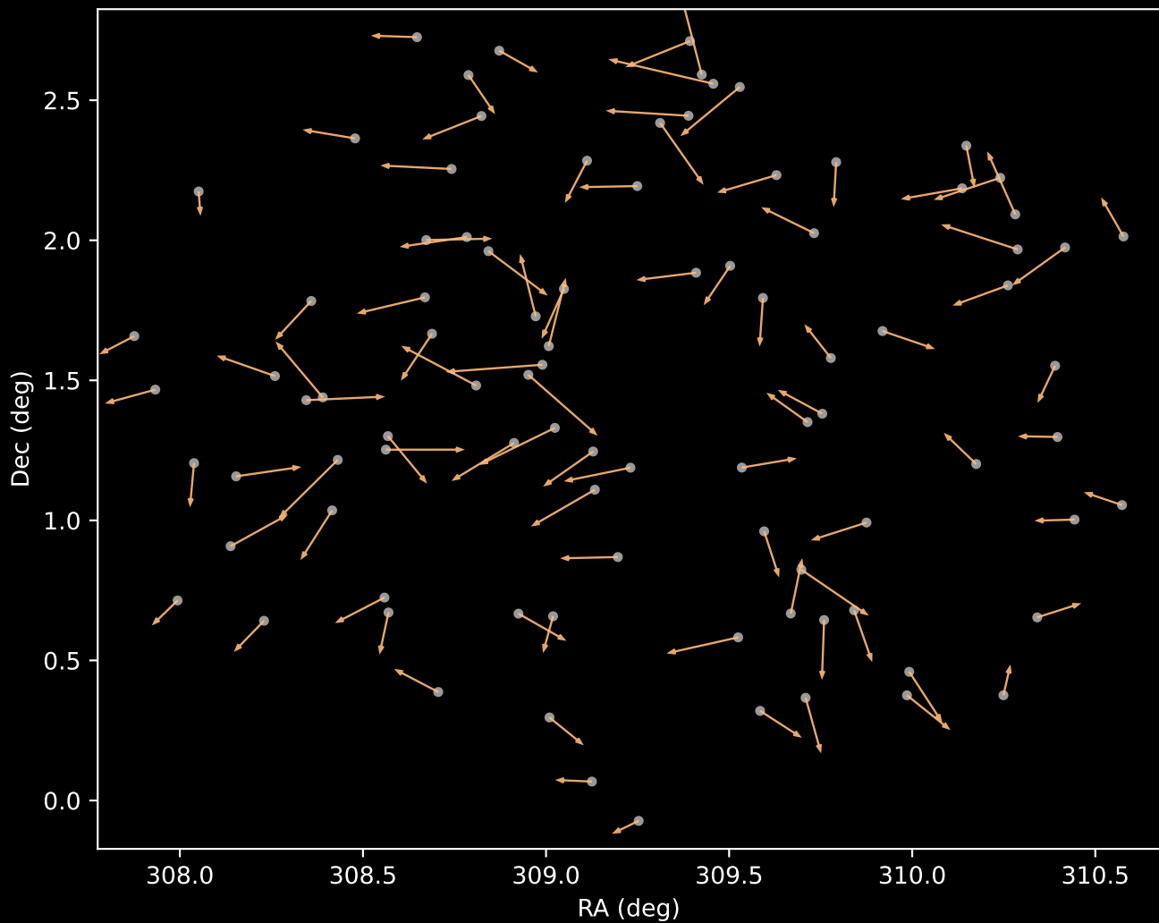
APOGEE DR17 Cluster 3 Proper Motion Vectors (n=92)
