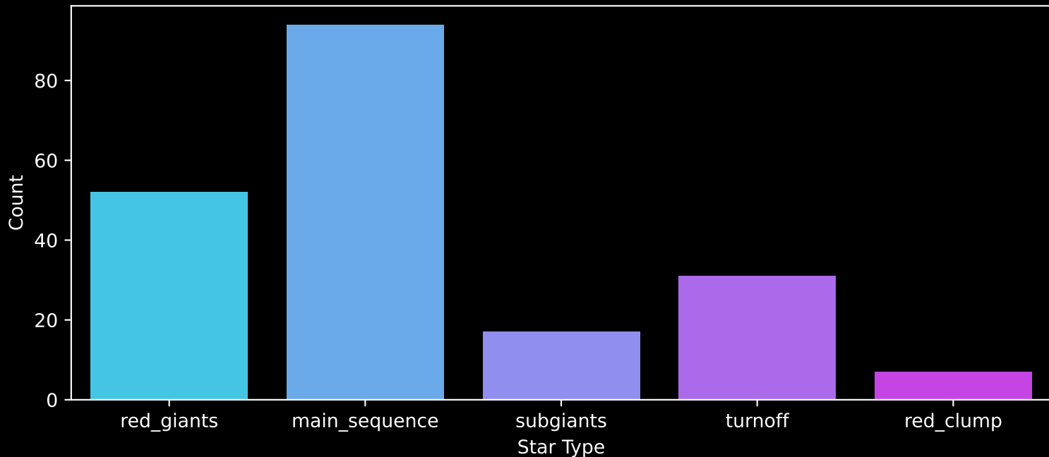
APOGEE DR17 Field: [337+60_MGA] Count plot of Star Type
