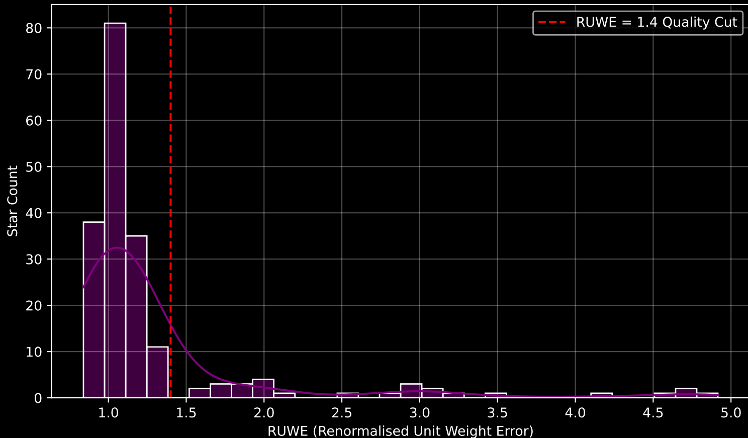
GAPOGEE DR17 Field [337+60_MGA] RUWE Distribution (n= 192)
