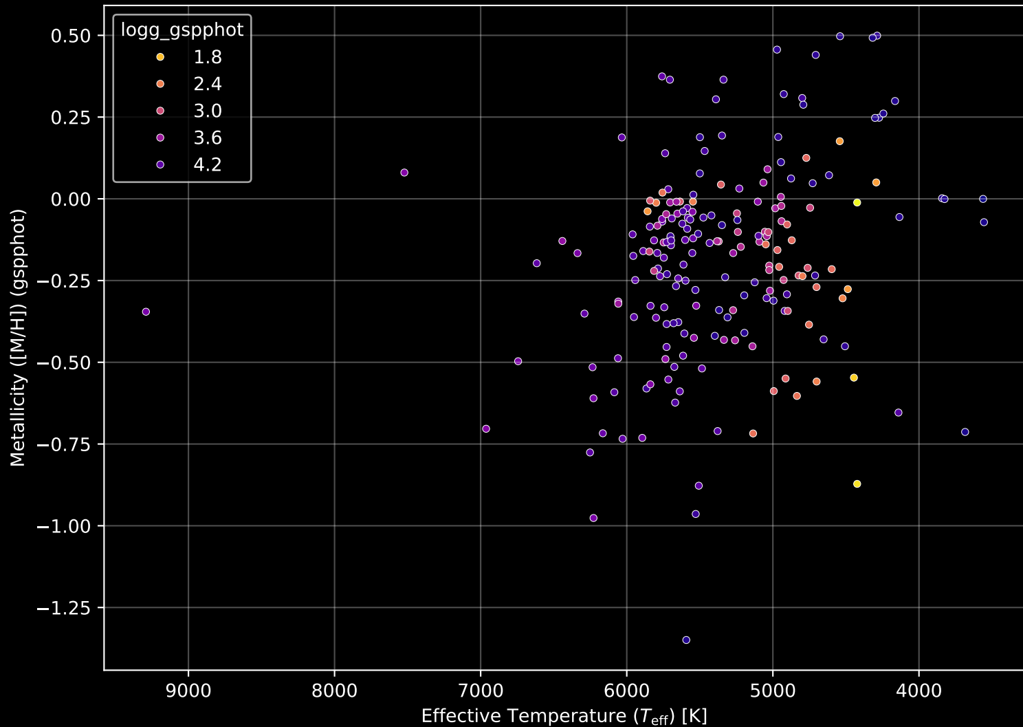
APOGEE DR17 Field: [337+60_MGA] Stellar Population Parameters (n= 201)
