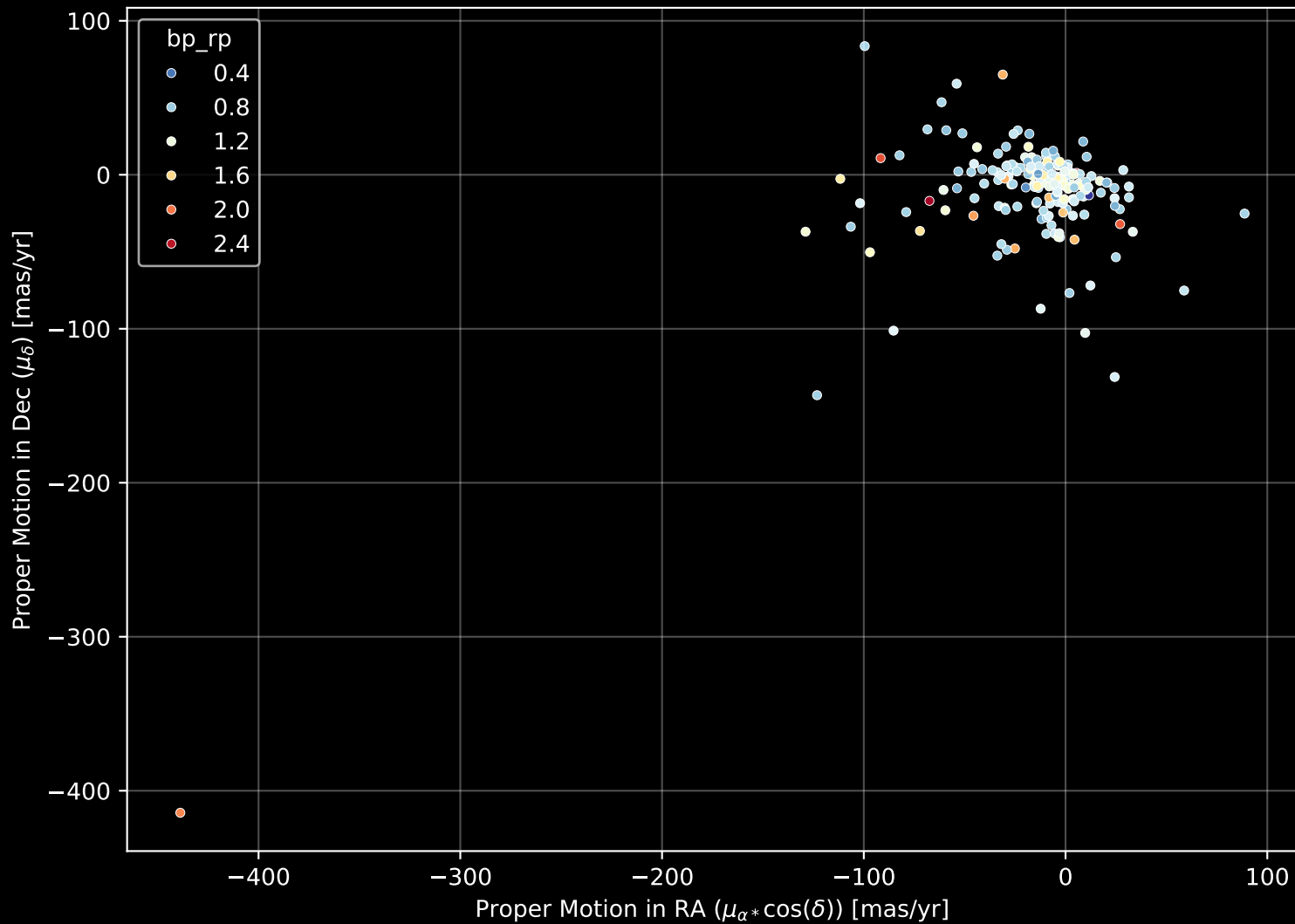
APOGEE DR17 Field: [337+60_MGA] Proper Motion Diagram (n= 201)
