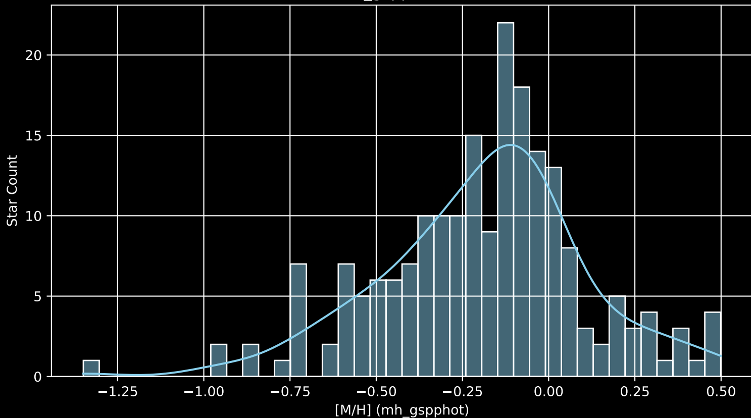
APOGEE DR17 Field: [337+60_MGA [M/H] (mh_gspphot) (n= 201)
