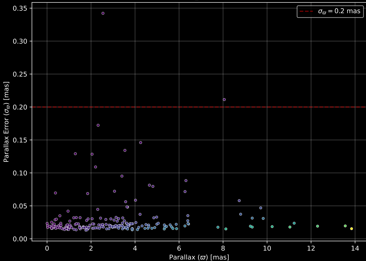
APOGEE DR17 Field: [337+60_MGA] Parallax Quality (n= 201)
